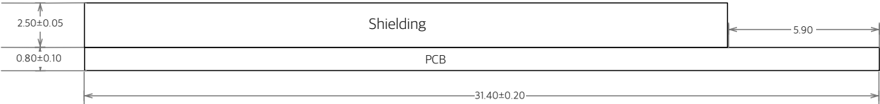
Figure 1: Top and Side View of ESP32-WROVER
